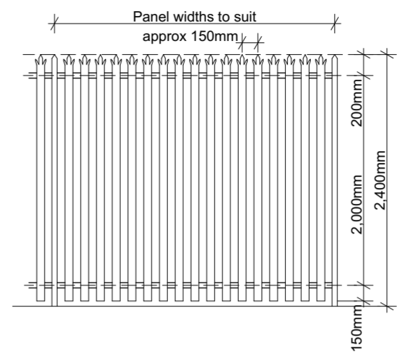
Fencing Elevation - 1:50 Palisade Fencing 2.4m high - Green RAL 6005
